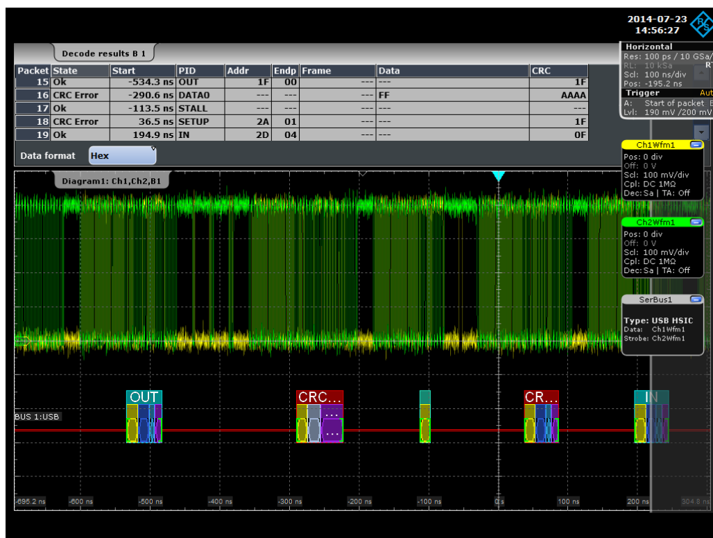
Figure 12-116: USB HSIC protocol: decoded and binary signal, and decode results
