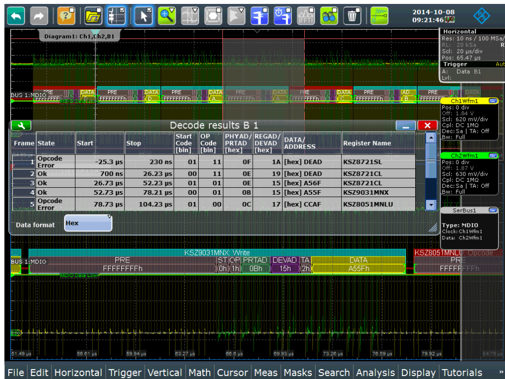
Figure 12-101: Decoded and binary MDIO signal trace, and decode results table
