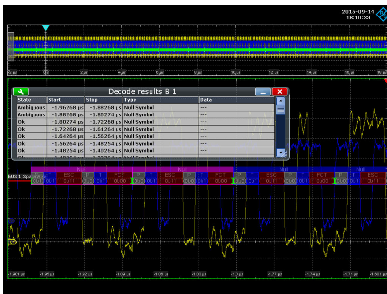
Figure 12-120: Decoded SpaceWire signal with ambiguous bits
