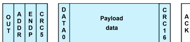
Figure 12-106: Example of a bulk OUT transfer. Blue: host speaks, white: device speaks
