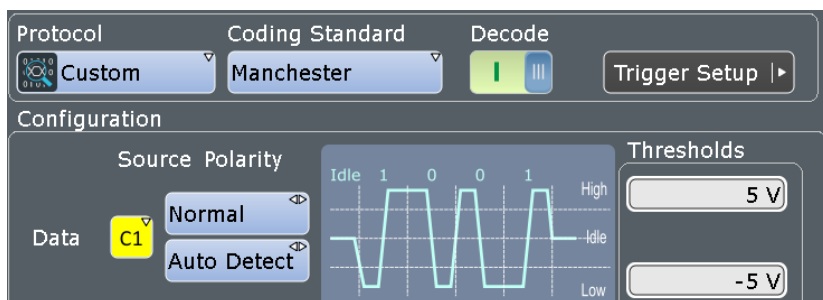
Figure 12-84: Custom serial bus coding configuration Manchester
