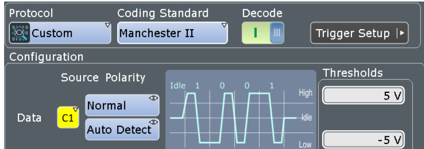
Figure 12-85: Custom serial bus coding configuration Manchester II
