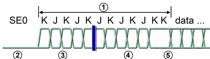
Figure 12-107: Start of a high speed packet: after an SE0, the packet starts with a SYNC field (or SOP), followed by the data packet
