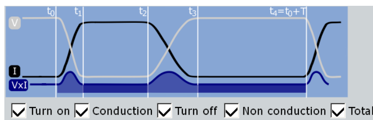
Figure 16-4: Switching loss phases
