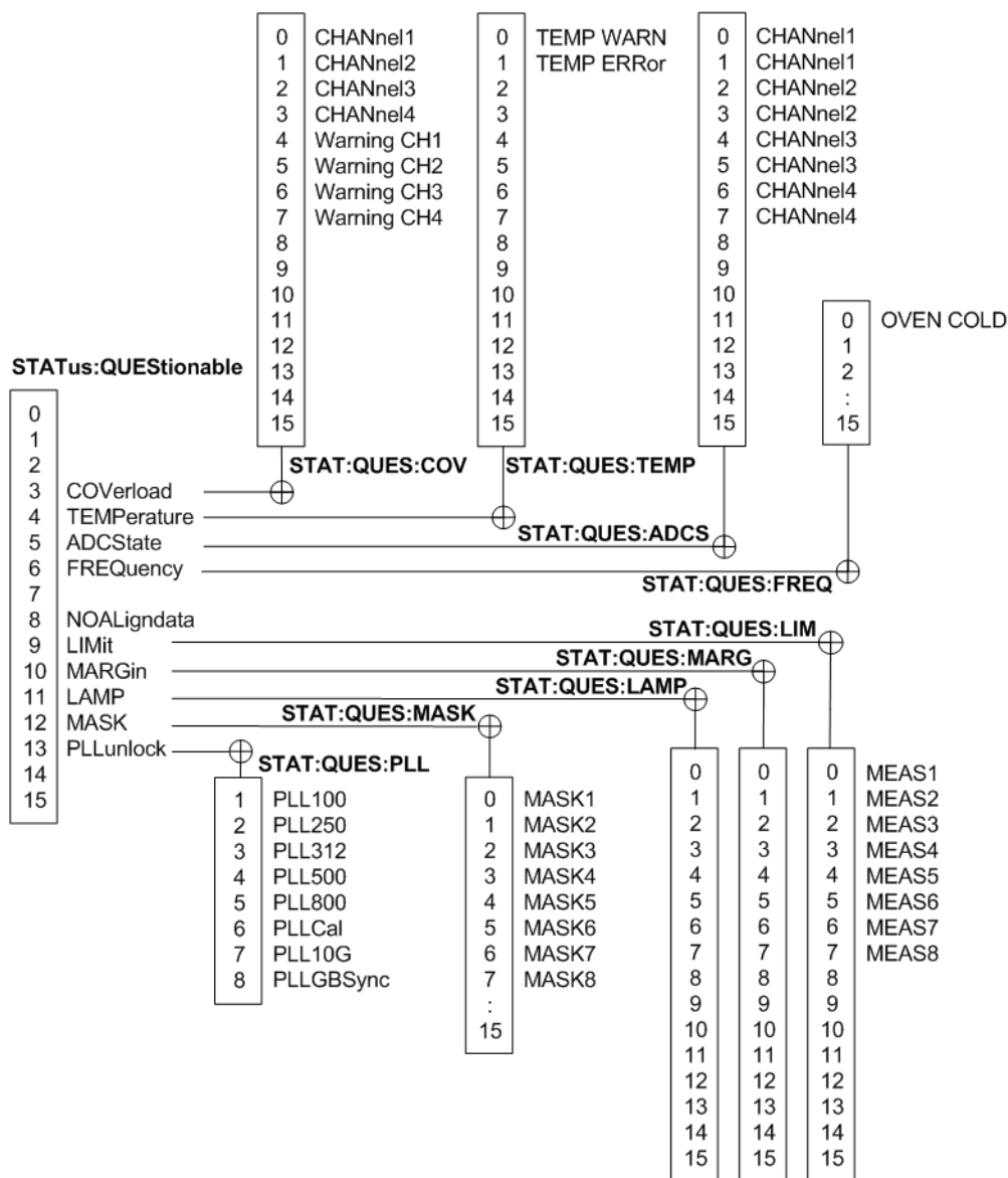
Figure 19-1: Overview of the STATus:QUESTionable register
