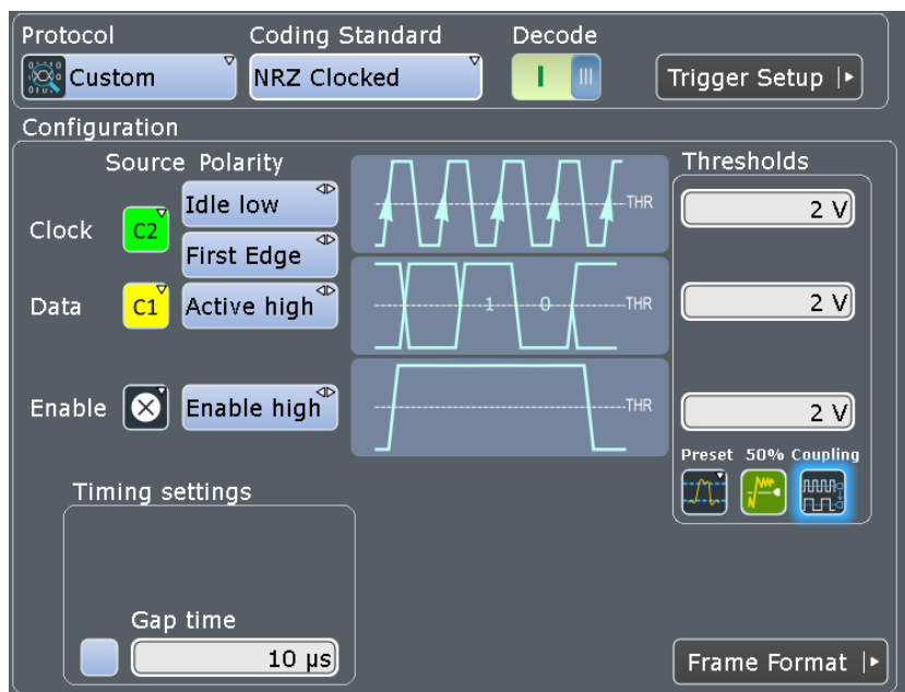
Figure 12-86: Custom serial bus coding configuration NRZ Clocked
