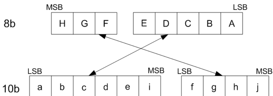
Figure 12-98: Coding scheme of the 8b/10b
