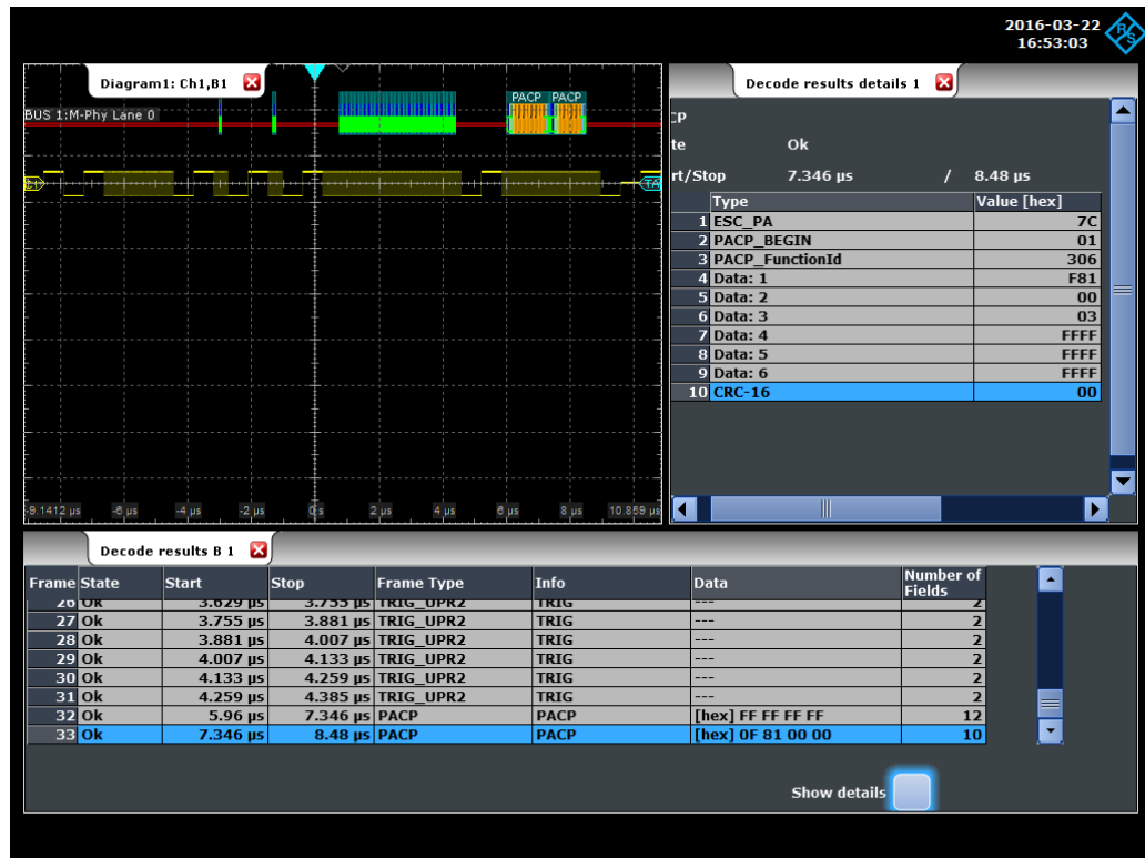
Figure 12-82: Decoded UniPro signal with result tables
