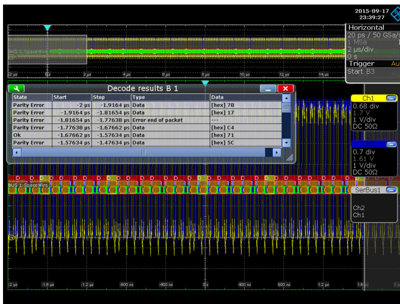
Figure 12-121: Decoded SpaceWire signal with a parity error
