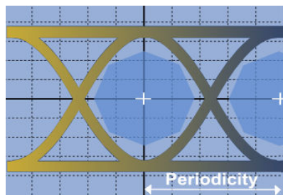
Figure 15-4: Eye mask with right periodicity
