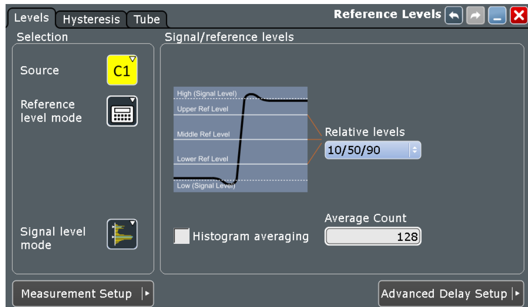
Figure 7-1: Automatic reference level definition
