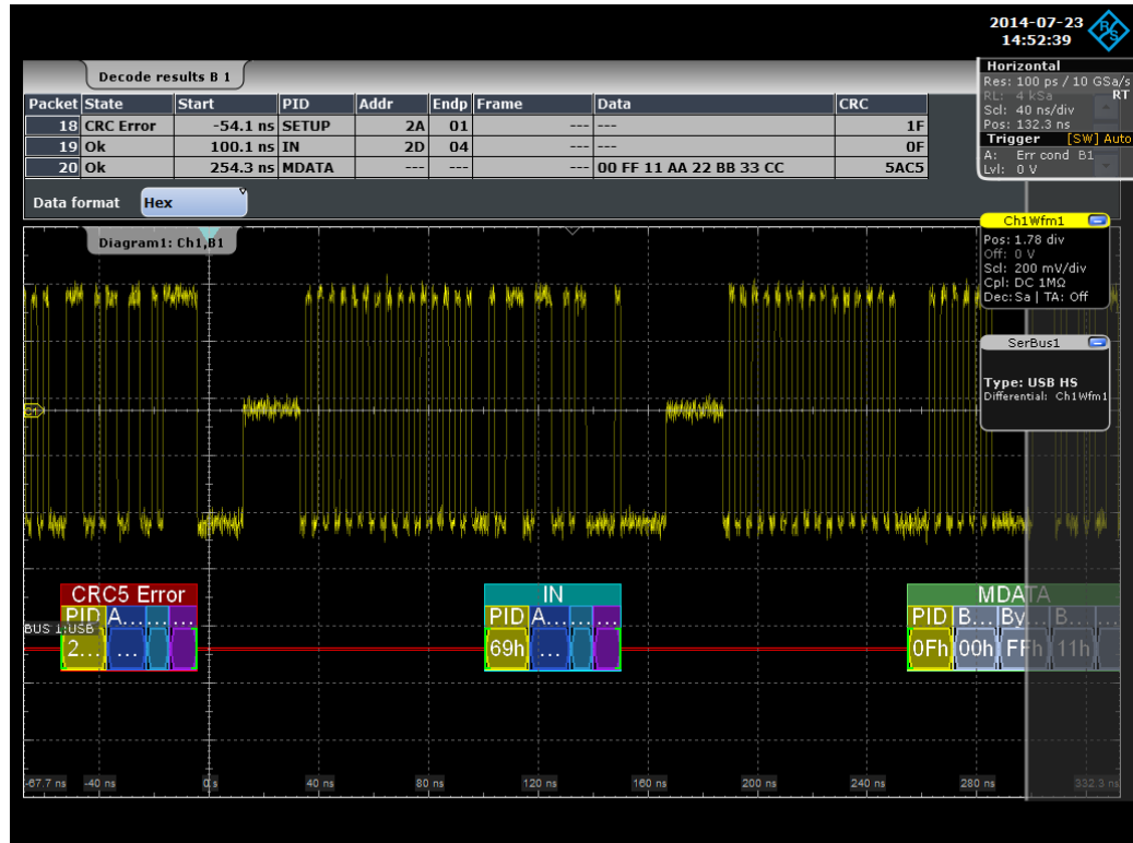
Figure 12-115: USB high speed protocol: decoded and binary signal, and decode results
