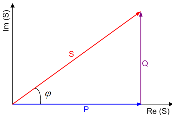
Figure 16-1: Power diagram for sinusoidal signals
