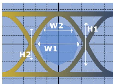
Figure 15-3: Main and minor widths and heights of an octagon eye mask
