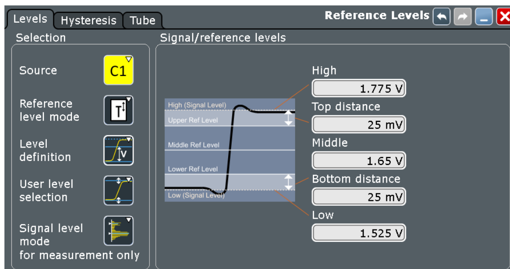
Figure 7-2: Manual reference level definition
