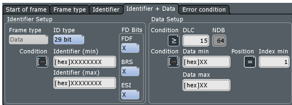
Figure 12-27: Identifier + Data search setup for CAN FD signals
