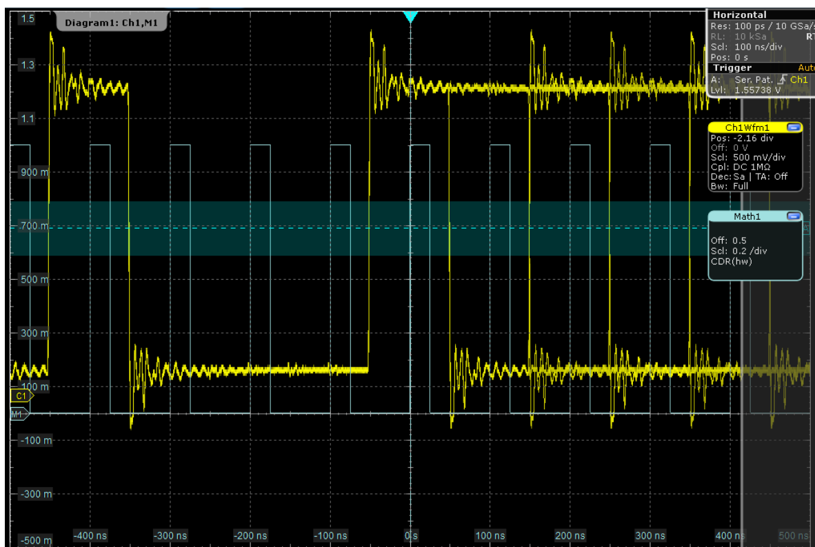
Figure 15-2: Data signal with 10 Mbps, serial pattern trigger on XXXX1000 with CDR and UI offset = 0.5, math waveform = CDR(hw)
